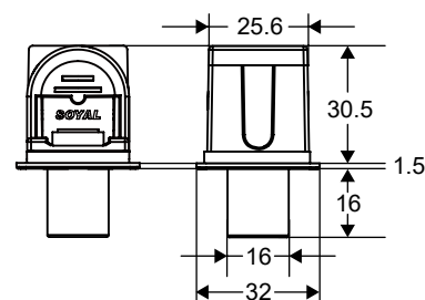
• Electric Bolt Lock Side View
